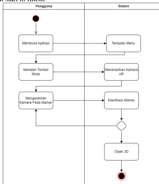
Fig. 2: Application's Activity Diagram
