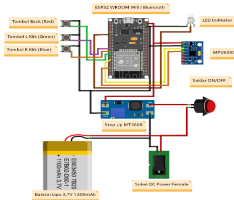
Figure 5: Hardware circuitry
