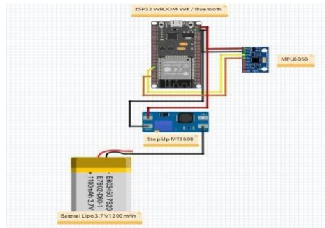
Figure 4: MT3608 Step Up Module & battery installation circuit
